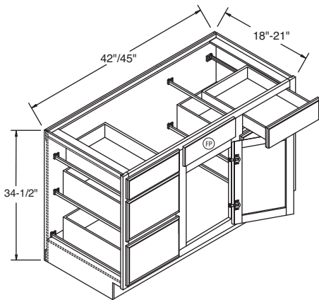
VBB4218DBH-VBB4518DBH L or R VBB42DBH-VBB45DBH L or R 6 drawers
