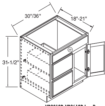
VB3018D-VB3618D L or R VB30D-VB36D L or R
