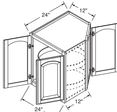
WPD2430S (WPD2430SRL shown)
