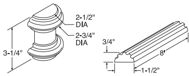
SPLIT SPOOL
