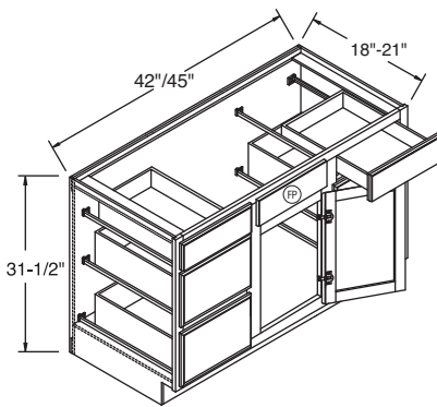
VBB4218D-VBB4518D L or R VBB42D-VBB45D L or R 6 drawers
