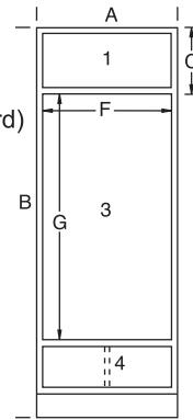
Single Oven Option 1
