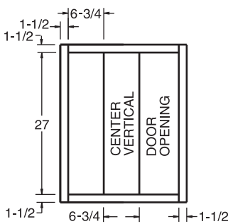
BLIND WALL CABINET
