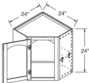
WD2424 L or R
