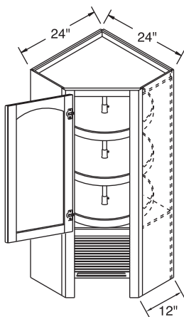
WDT2457S-WDT2460S L or R
