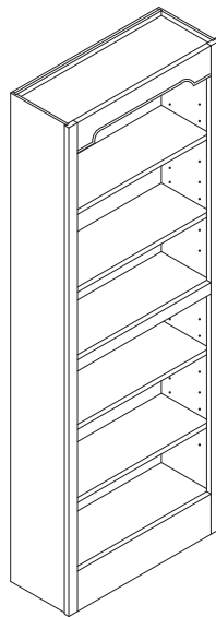
Shelf Units: Custom front frames can be built with arched, furniture or frieze valance top rails. Specify the bottom of the unit with a flush toe kick (field applied furniture base moulding) and matching interior. Maximum width of 36" and height of 96". One fixed shelf. Enhance the open shelf unit with cabinet doors. Field applied Soffit A moulding to any of the shelves creates a plate rail.
