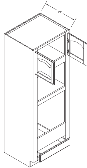
Custom Appliance Cabinet: Using your appliance specifications, create a custom microwave/oven unit from a universal oven cabinet.
