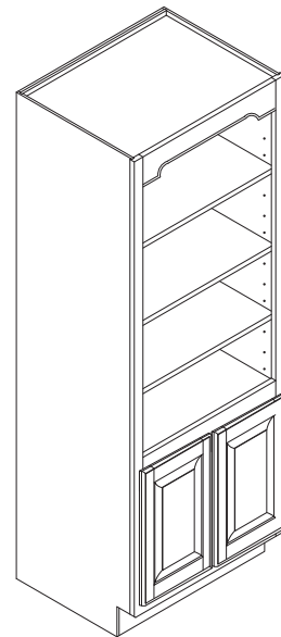
Shelf Units: Custom front frames can be built with arched, furniture or frieze valance top rails. Specify the bottom of the unit with a flush toe kick (field applied furniture base moulding) and matching interior. Maximum width of 36" and height of 96". One fixed shelf. Enhance the open shelf unit with cabinet doors. Field applied Soffit A moulding to any of the shelves creates a plate rail.
